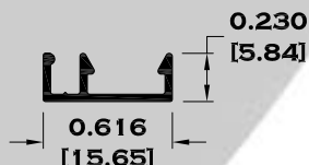
5377 MOSQUITERO
