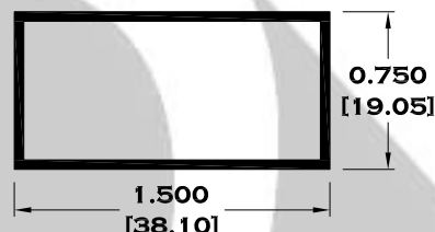
11086 TUBO RECTANGULAR DE 1 1/2" X 3/4"
