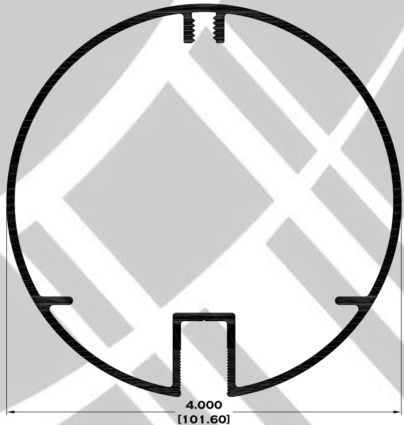
2840 PASAMANOS REDONDO 4"
