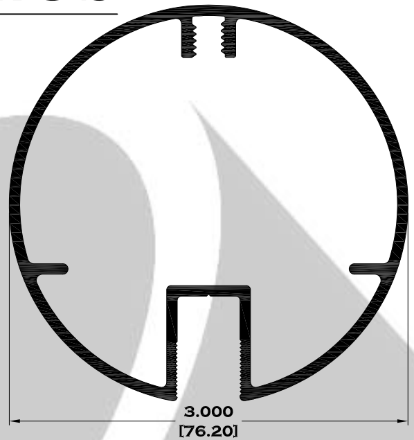
2830 PASAMANOS REDONDO 3"
