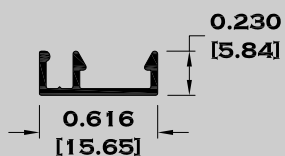
5377 MOSQUITERO LIGERO
